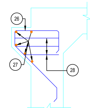
BRACKET REINF. DETAIL (SCALE-1:30)
