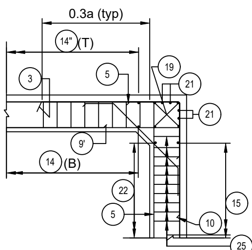
DETAIL-2 (SCALE-1:40)
