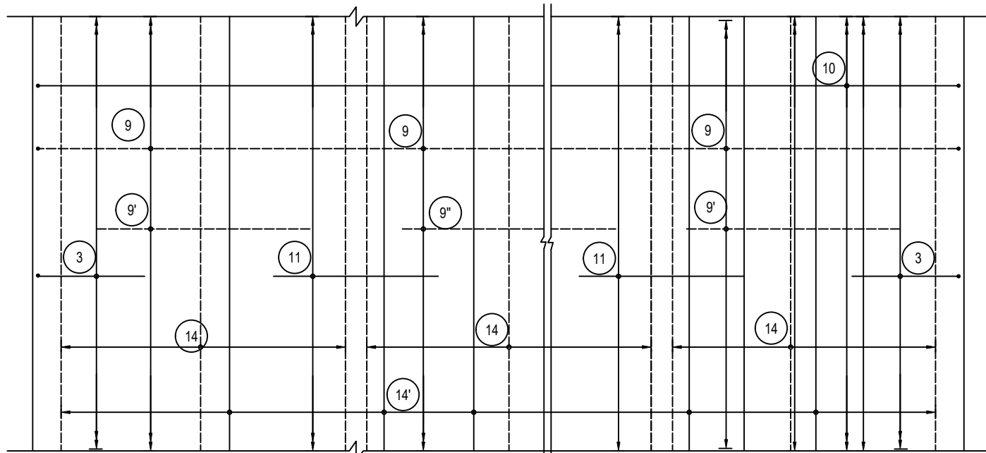
REINFORCEMENT DETAILS OF TOP SLAB HAUNCH BAR NOT SHOWN IN PLAN FOR CLARITY
