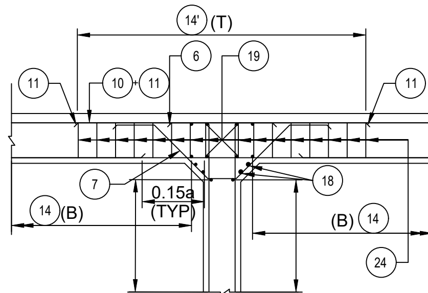
DETAIL-4 (SCALE-1:40)
