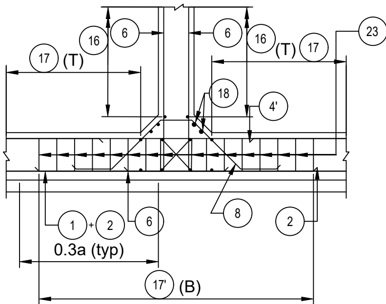
DETAIL-3 (SCALE-1:40)
