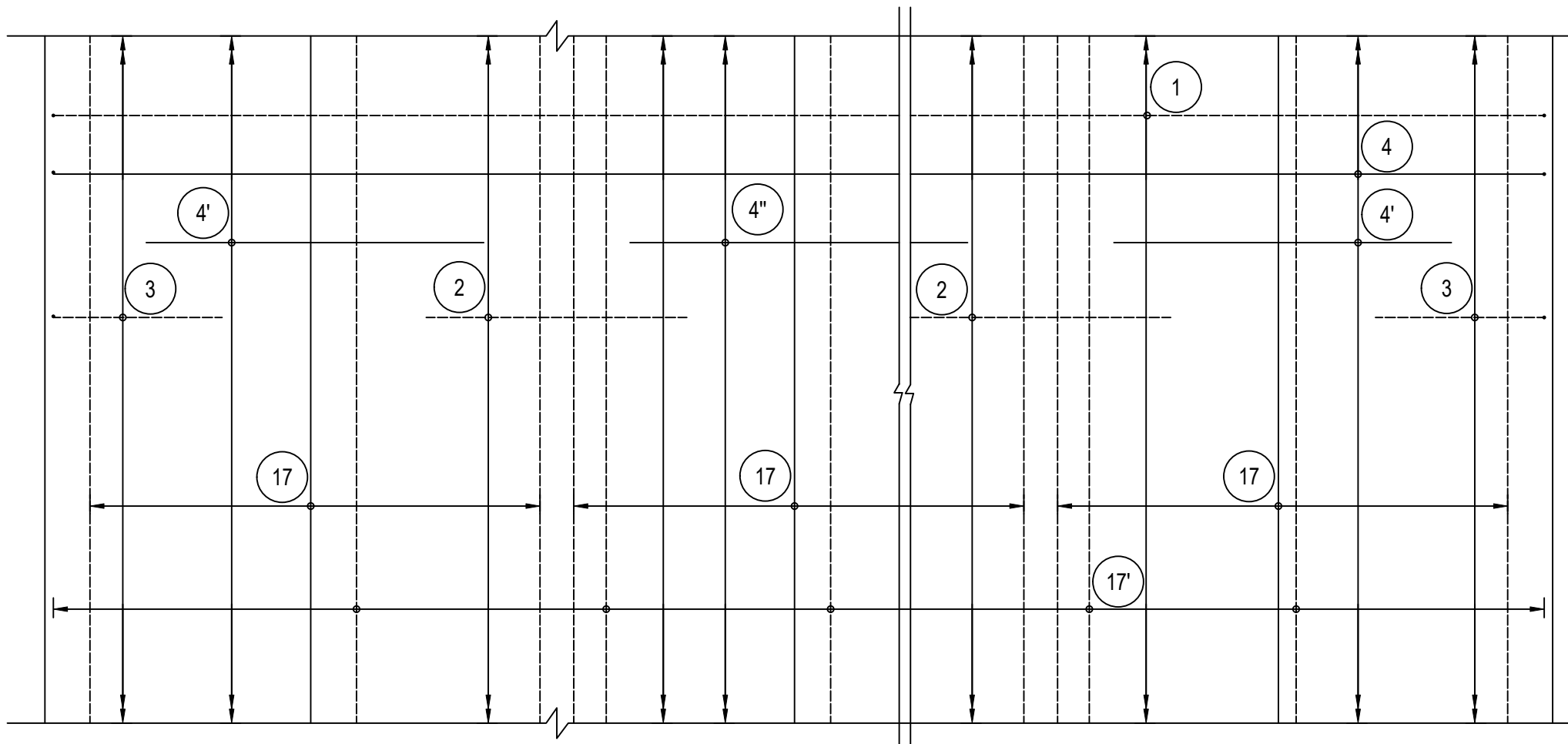
REINFORCEMENT DETAILS OF BOTTOM SLAB HAUNCH BAR NOT SHOWN IN PLAN FOR CLARITY
