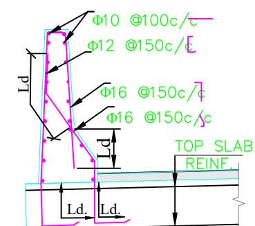
REINFORCEMENT DETAIL OF CRASH BARRIER (SCALE 1:40)
