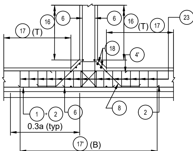
DETAIL-3 (SCALE-1:40)
