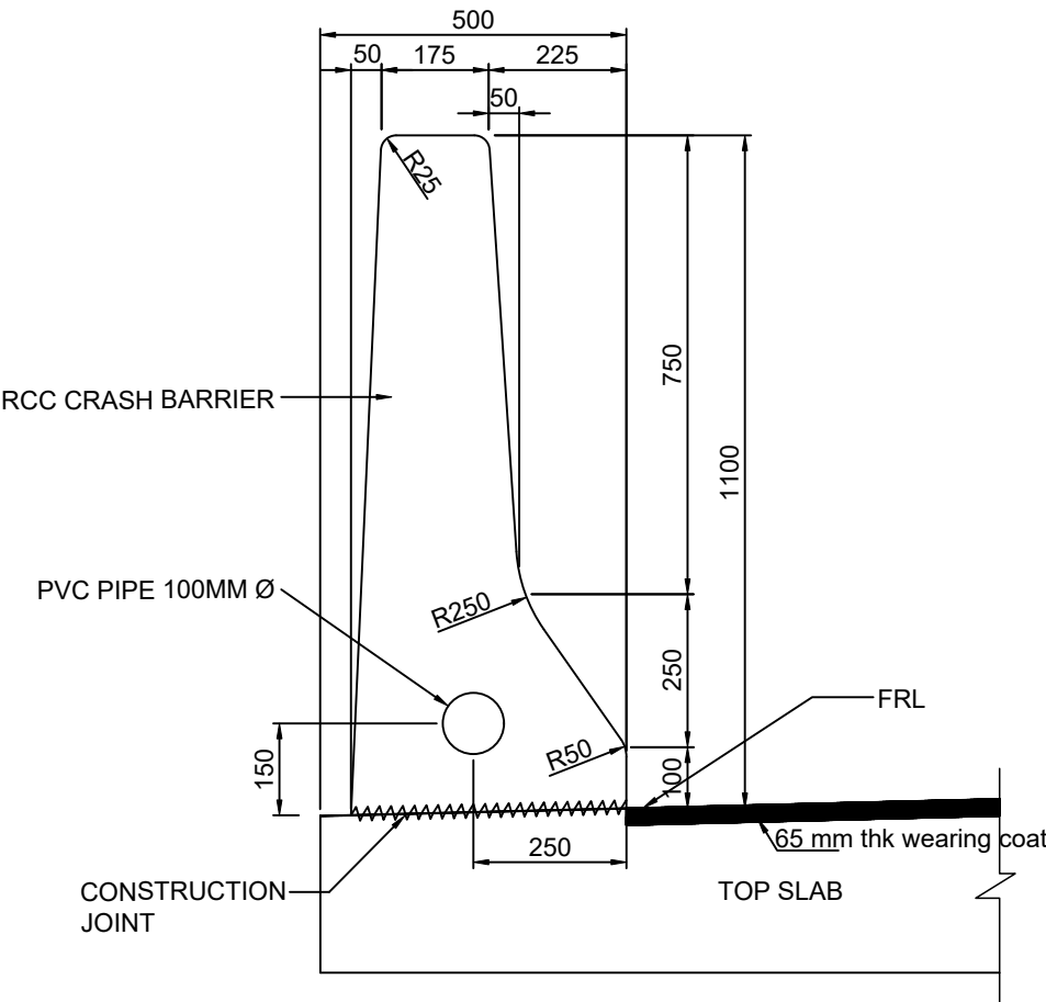
DIMENSION DETAIL OF CRASH BARRIER WITHOUT FOOTPATH (SCALE 1:10)
