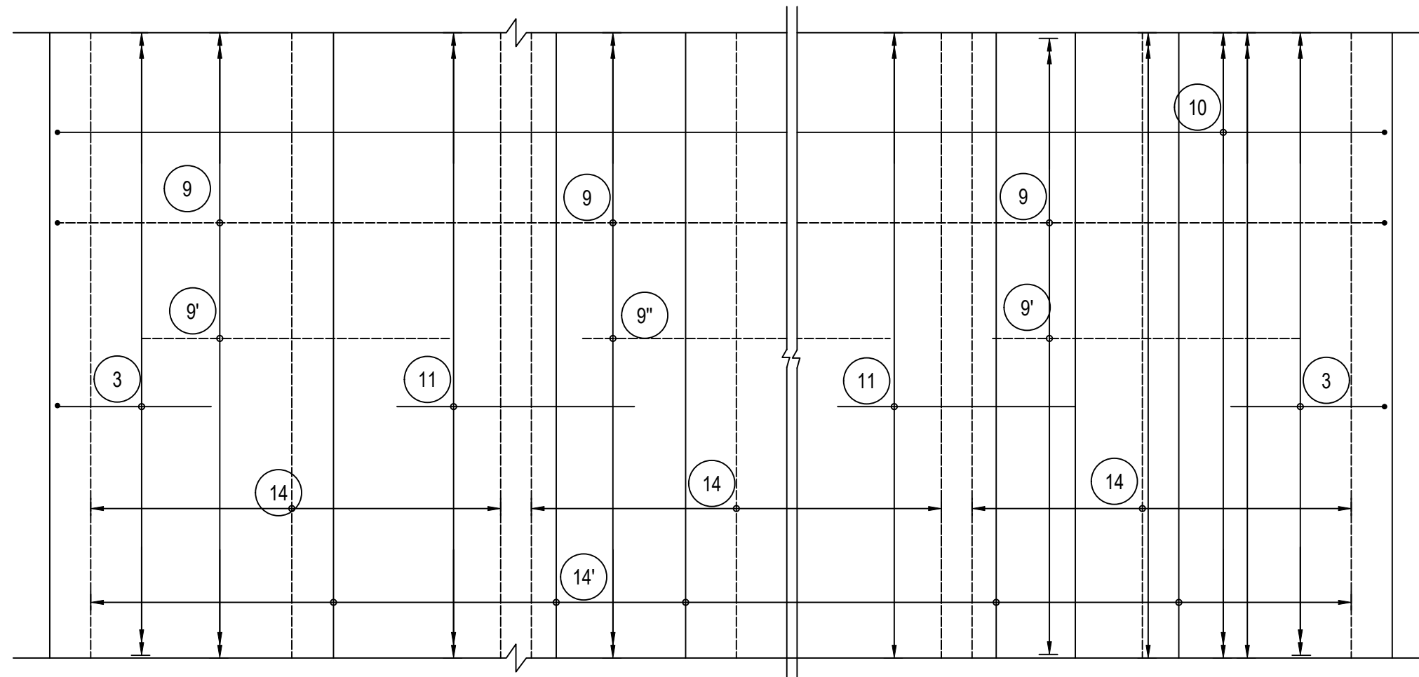
REINFORCEMENT DETAILS OF TOP SLAB HAUNCH BAR NOT SHOWN IN PLAN FOR CLARITY
