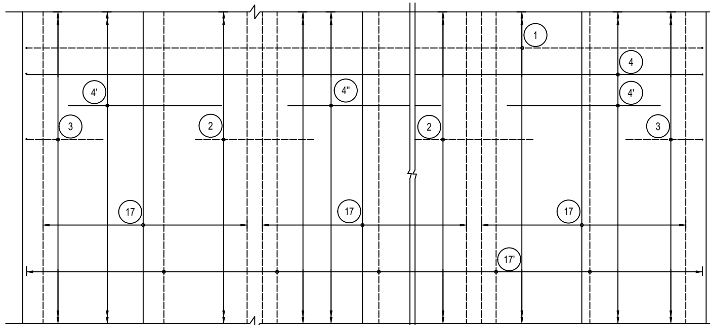
REINFORCEMENT DETAILS OF BOTTOM SLAB HAUNCH BAR NOT SHOWN IN PLAN FOR CLARITY
