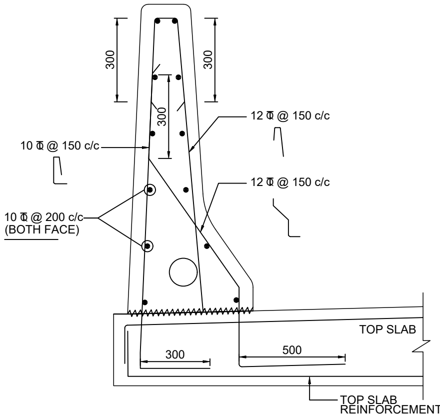
REINFORCEMENT DETAIL OF CRASH BARRIER WITHOUT FOOTPATH (SCALE 1:10)
