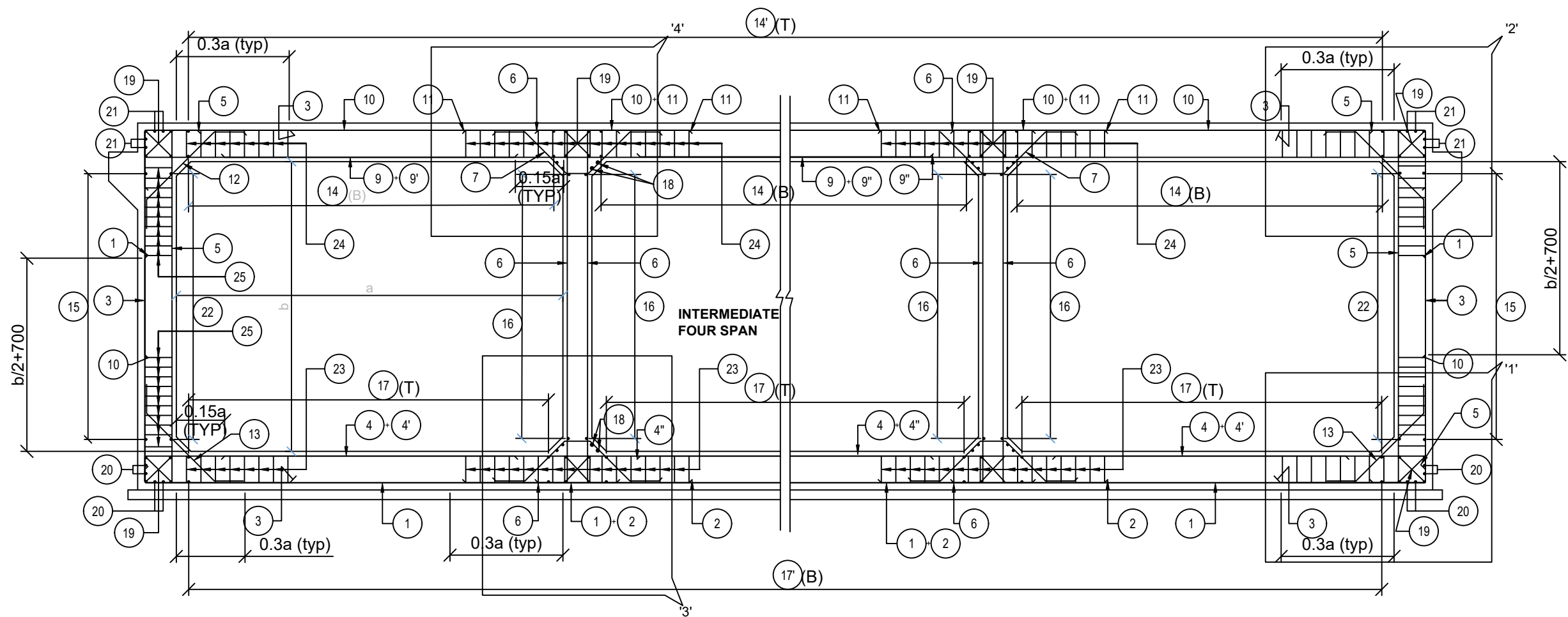
LONGITUDINAL SECTION OF BOX STRUCTURE
