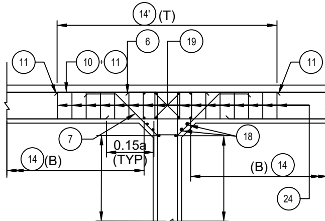
DETAIL-4 (SCALE-1:40)
