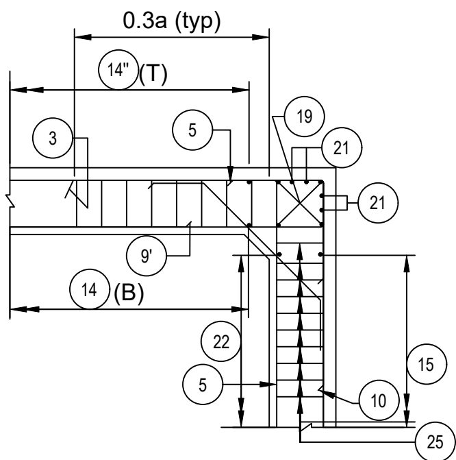
DETAIL-2 (SCALE-1:40)
