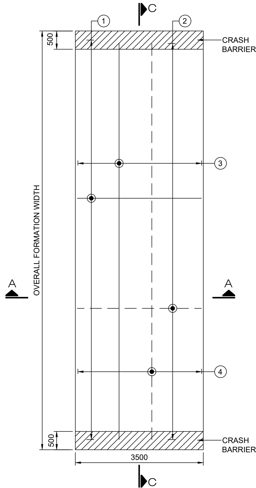
P L A N RC DETAILS OF APPROACH SLAB WITHOUT FOOTPATH (SCALE:-1:50)
